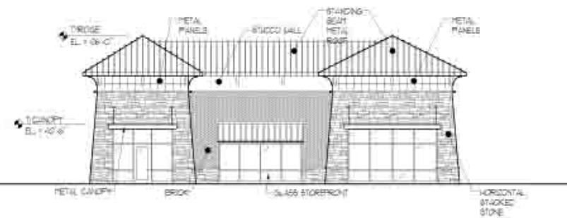
SOUTH ELEVATION
