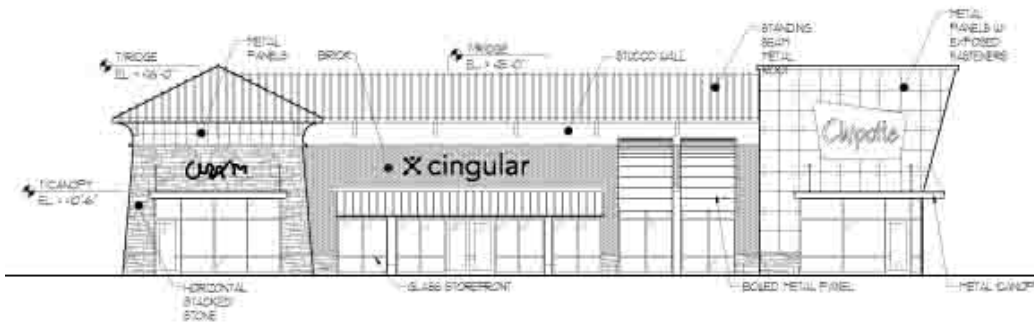
EAST ELEVATION
